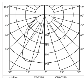
Light distribution LED 10.9 W.
