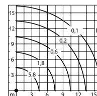
Light distribution LED 19 W.
