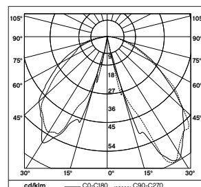
Light distribution LED 6 x 2.4 W.
