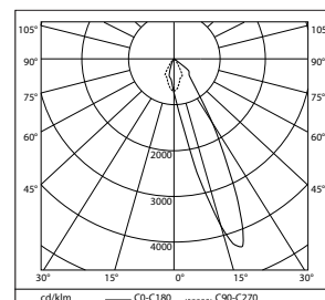
Light distribution LED 5.4 W.
