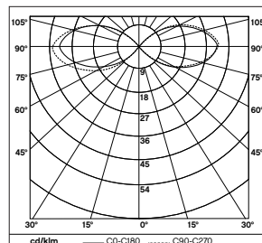
Light distribution LED 10 W.
