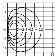
Light distribution LED 7.2 W.
