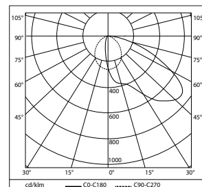
Light distribution LED 21.5 W.
