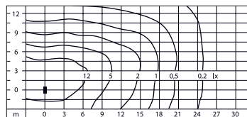
Light distribution LED 45 W.
