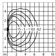
Light distribution LED 7 W.
