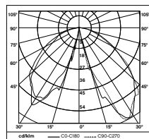
Light distribution 16.8 W
