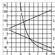
Light distribution 19 W
