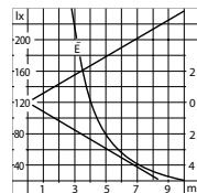
Light distribution 40 W
