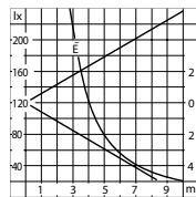
Light distribution 40 W
