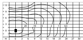
Light distribution 33.5 W
