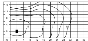
Light distribution 51.2 W
