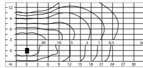
Light distribution 33.5 W
