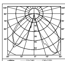
Light distribution 16.8 W
