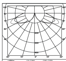
Light distribution 14.1 W
